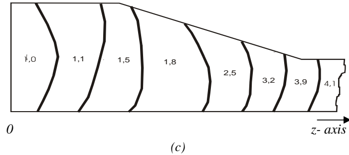
Figure 3. The contours of axial velocity v_a [mm/s] ( v_{punch} = 12 mm/s, R_{area} = 73\% ) for: (a) coefficient of friction \mu = 0,05 ; (b) coefficient of friction \mu = 0,11 ; (c) coefficient of friction \mu = 0,16
