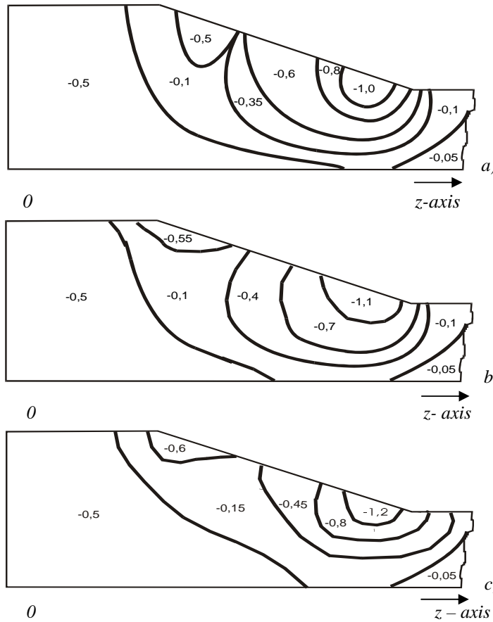
Figure 4. The contours of radial velocity v_r [mm/s] ( v_{punch} = 12 mm/s, R_{area} = 73\% ) for: (a) coefficient of friction \mu = 0,05 ; (b) coefficient of friction \mu = 0,11 ; (c) coefficient of friction \mu = 0,16
