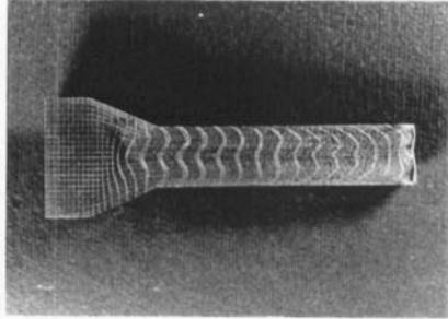
Figure 2. Deformed grid on the cold extruded alloy ( \mu=0,05 , v_{punch} = 12\text{mm/s} , R_{area} = 73\% ).
